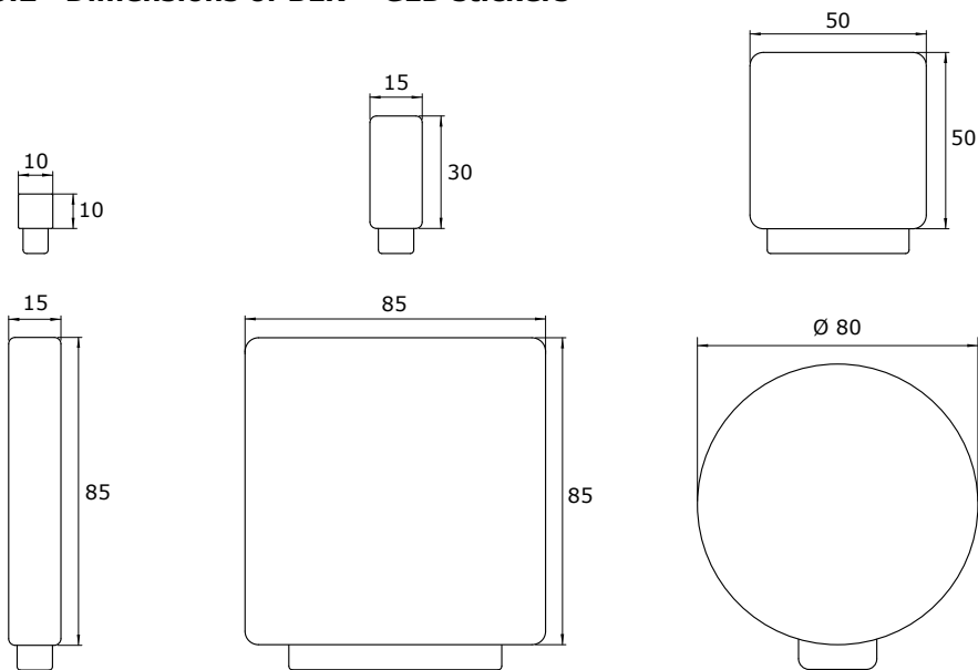
Figure 5.2.1 Dimensions of BLK – GLD sticker series; all dimensions in \times 10^{-3} m for both BLK and GLD sticker. Top row from left to right: -10X10, -15X30, -50X50. Bottom row from left to right: -15X85, -85X85 and -80. All BLK stickers have a thickness of 0.14 mm, GLD stickers have a thickness of 0.05 mm.
