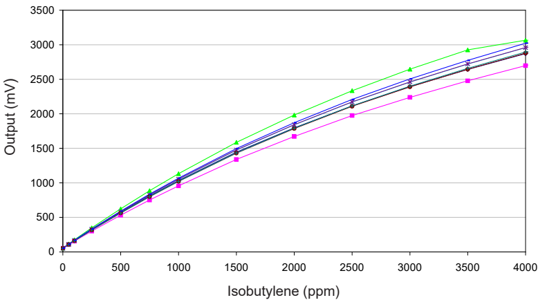
Figure 2 Linearity to Isobutylene
